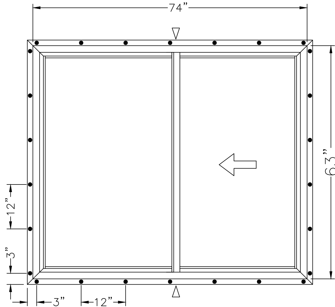
1630 HORIZONTAL SLIDING WINDOW (XOX) – FIN INSTALLATION MAXIMUM SIZE 110" X 63" DESIGN PRESSURE +/- 50 PSF MISSILE D – WIND ZONE 3
