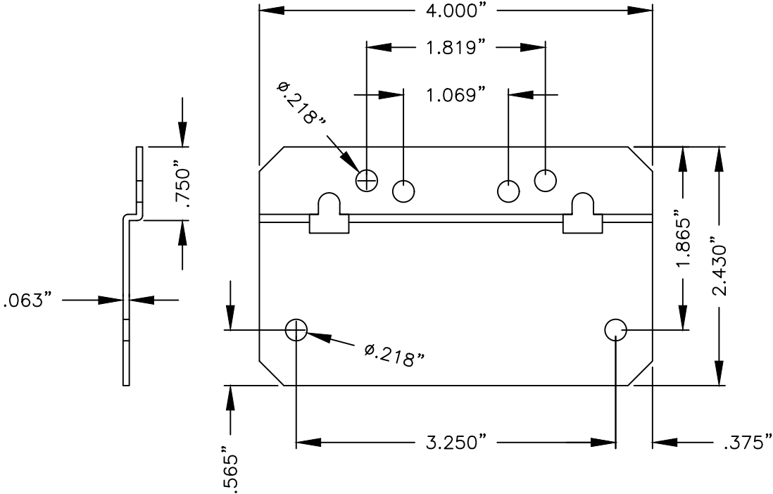
HD000063 ANCHOR STRAP COLD ROLLED STEEL (GALVANIZED)
